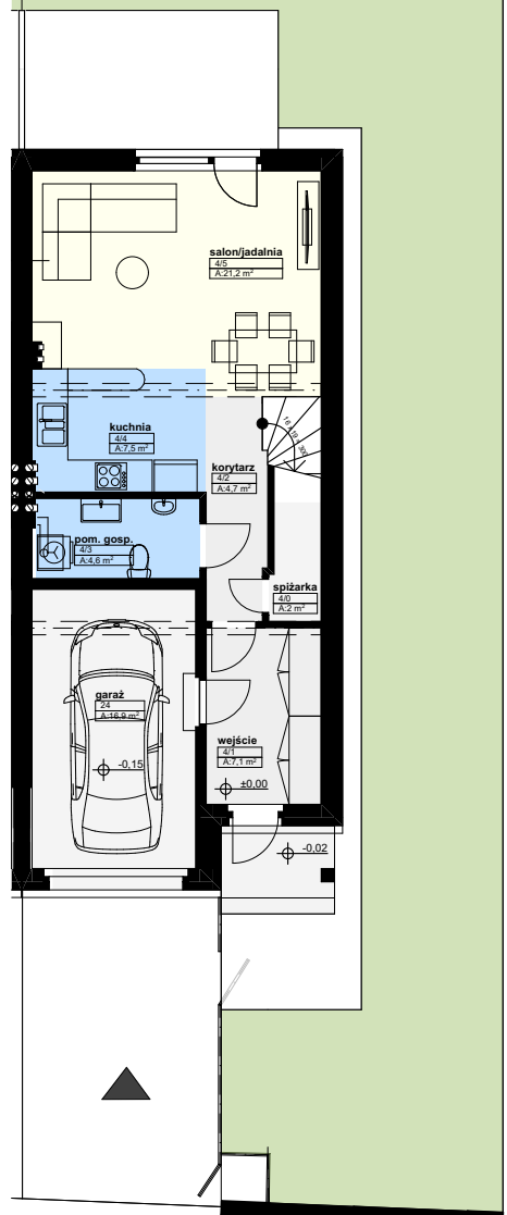
PARTER 0
