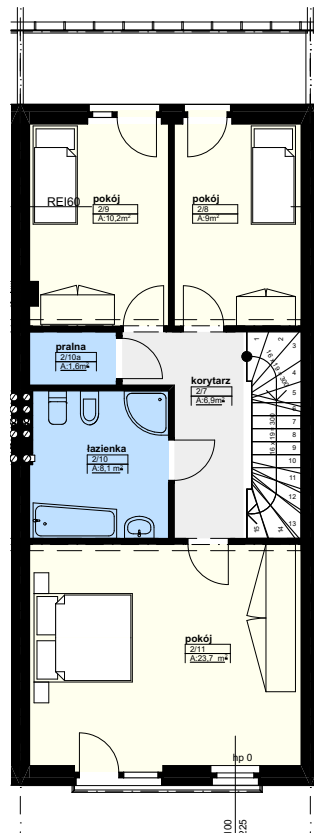
PIĘTRO +1
