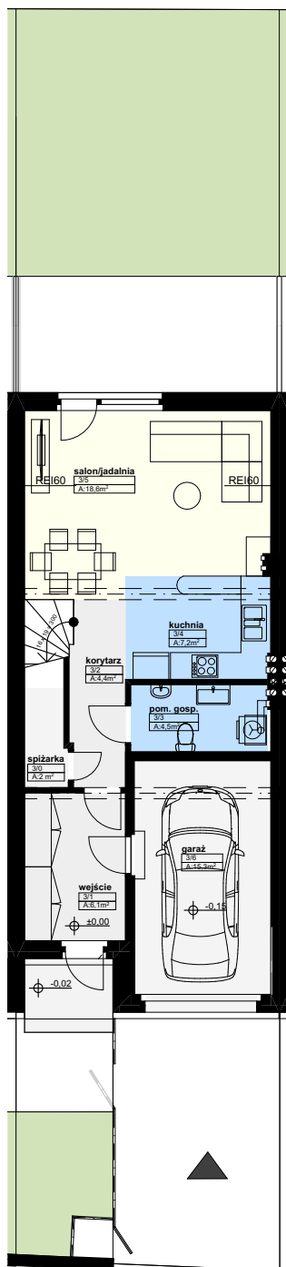
PARTER 0
