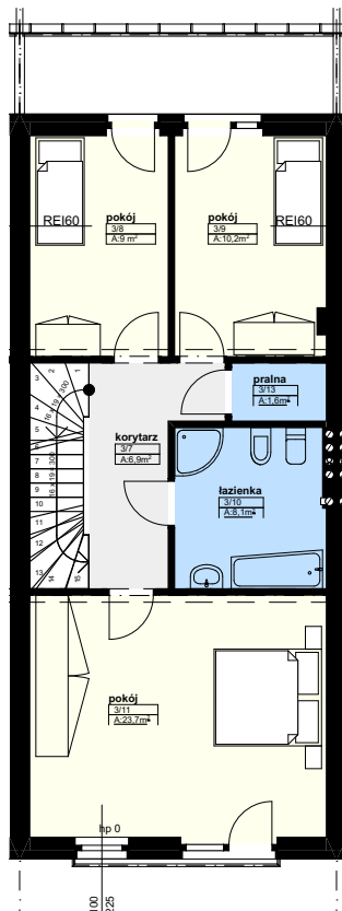
PIĘTRO +1
